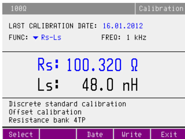
Figure 13 Offset calibration
