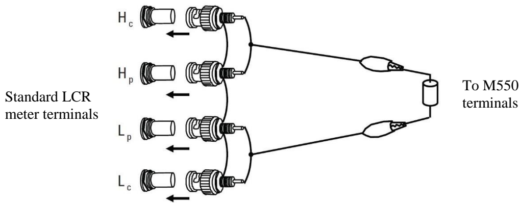
Figure 11 Standard LCR meter connection for 2W capacitance standard verification
