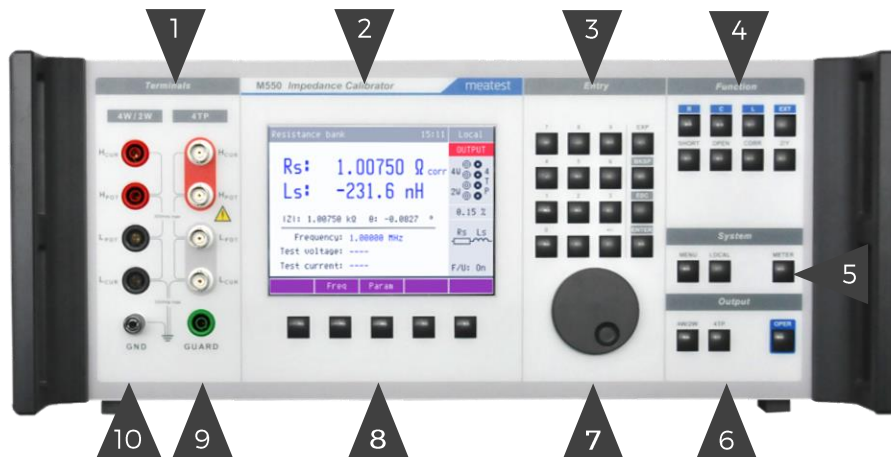
Figure 1 Front panel
