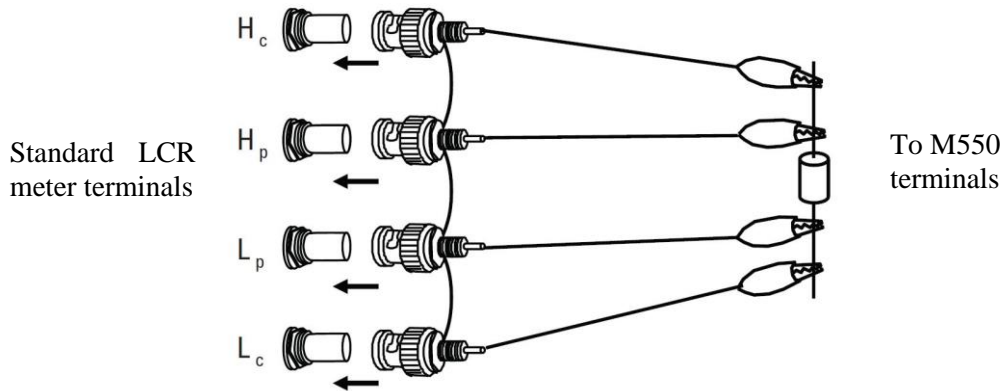
Figure 10 Standard LCR meter connection for 4W capacitance standard verification
