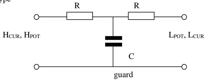
Figure 5 T inductance network
