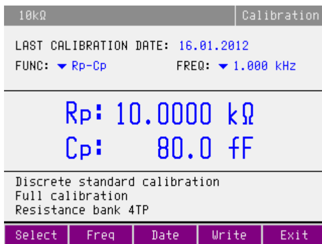
Figure 14 Full calibration
