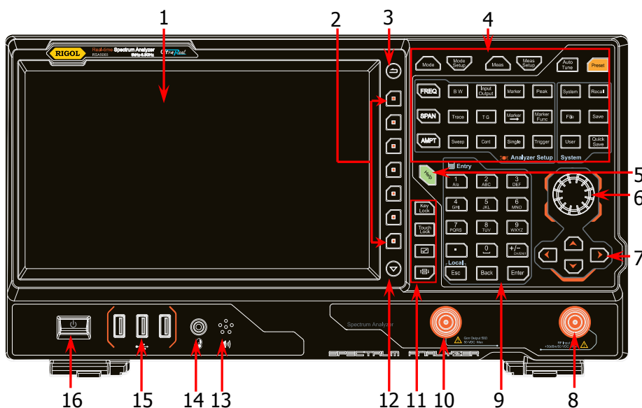
Figure 1-4 Front Panel
