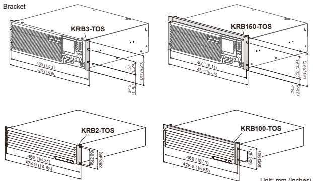
Bracket
