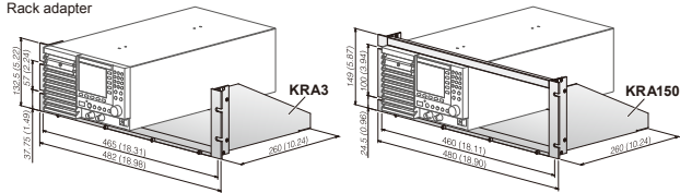
Rack adapter
