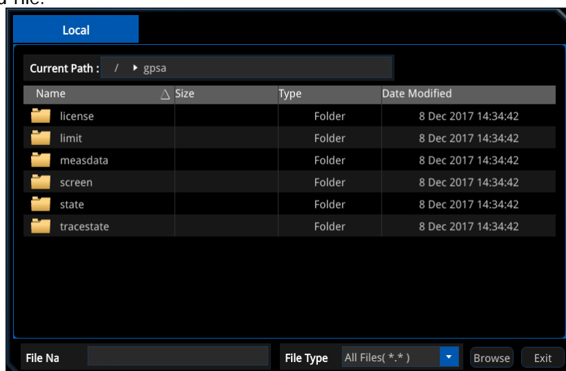
Figure 3-11 File Manager
