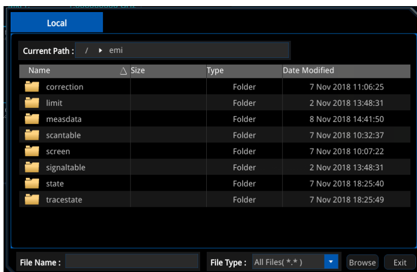
Figure 4-5 File Manager
