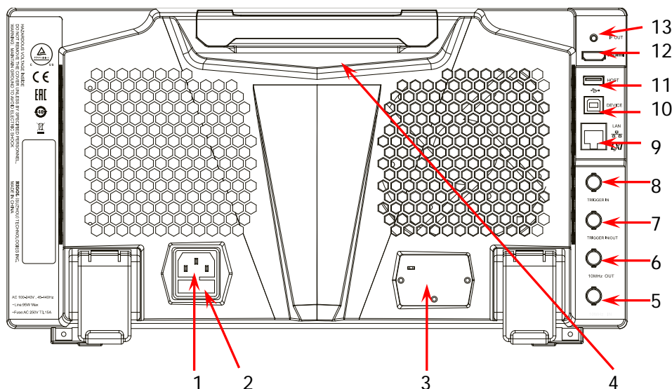
Figure 1-8 Rear Panel
