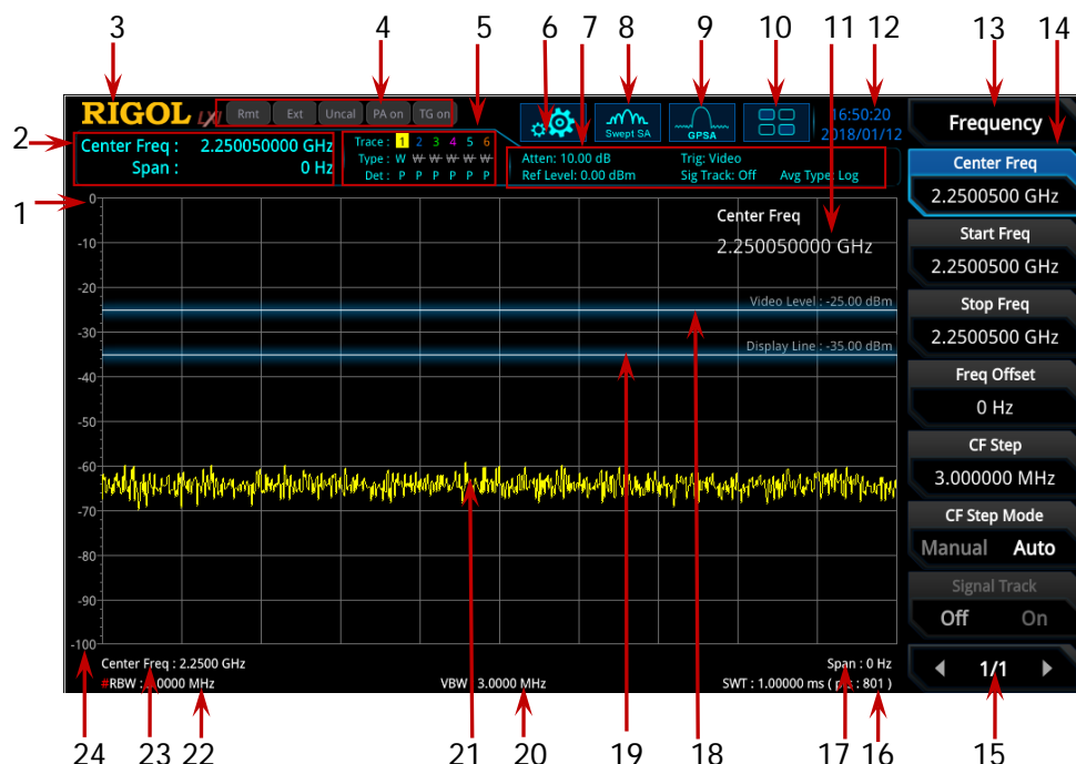
Figure 1-9 User Interface
