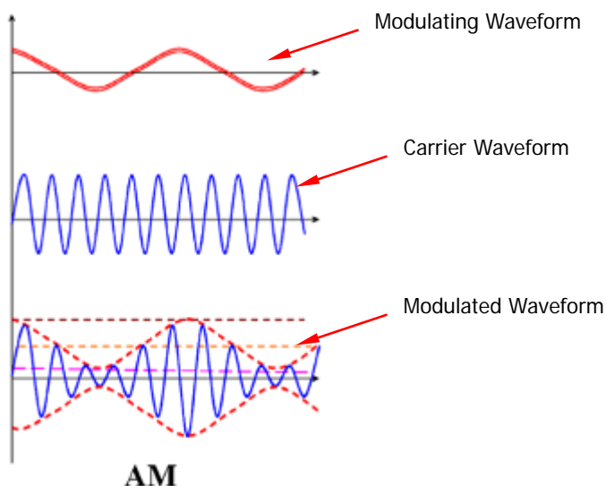
Figure 13-9 Amplitude Modulation
