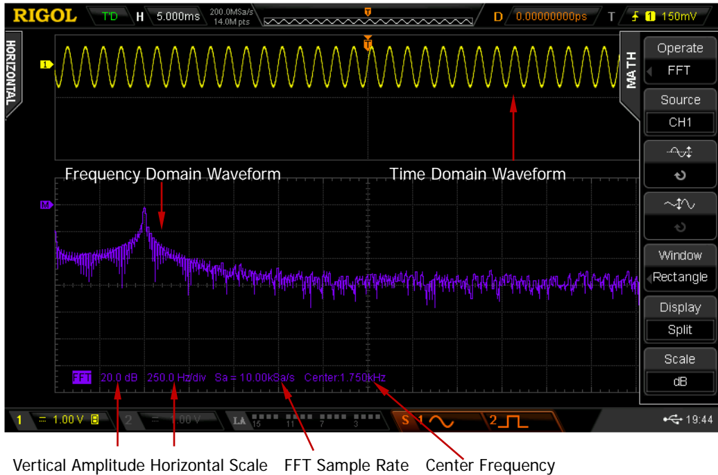
Figure 6-1 FFT Operation
