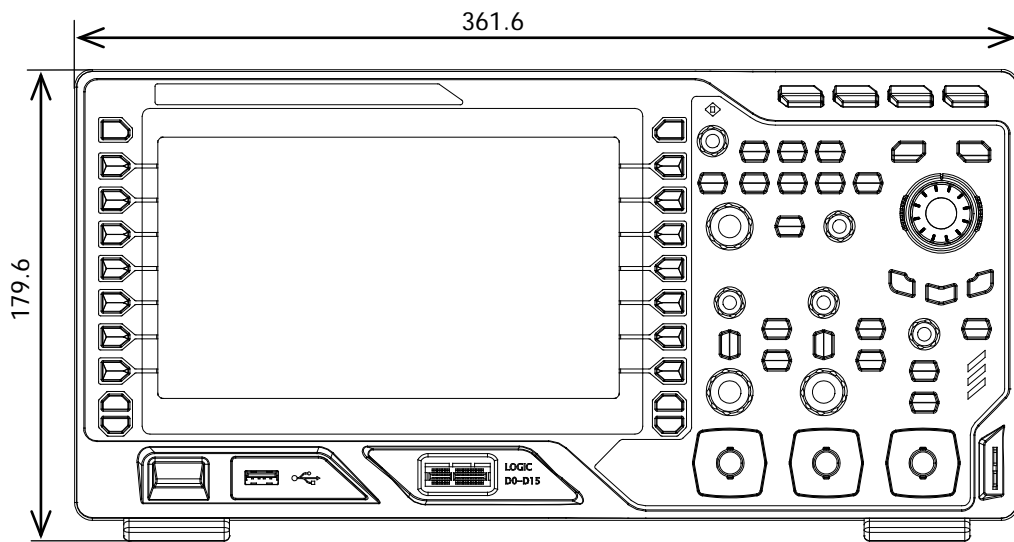
Figure 1-1 Front View
