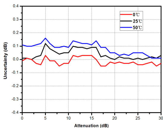
Measured ATT Switching Uncertainty VS temperature of DSA832E
