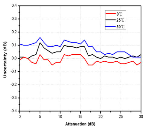
Measured ATT switching uncertainty VS temperature of DSA815/DSA832/DSA875
