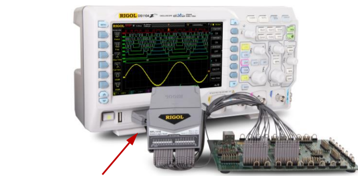
Figure 1-6 To Connect the Logic Probe
