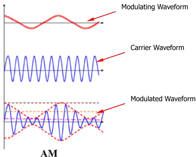
Figure 13-10 Amplitude Modulation
