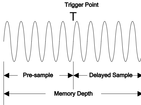
Figure 4-3 Memory Depth
